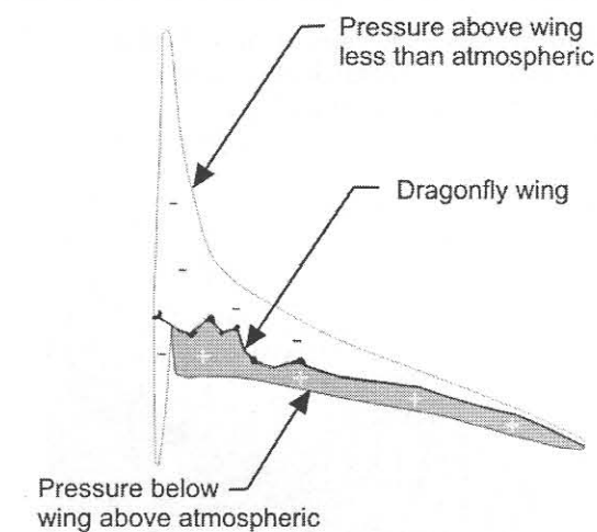
Figure 1. Pressure distribution over dragonfly wing cross section. The wing is at an angle of attack, so the pressure near the leading edge is below atmospheric both below and above the wing, but is much lower above the wing, so the net pressure is upward. On the remainder of the wing (roughly the subcosta to the trailing edge), the pressure below the wing is above atmospheric, while that above the wing is below atmospheric.
