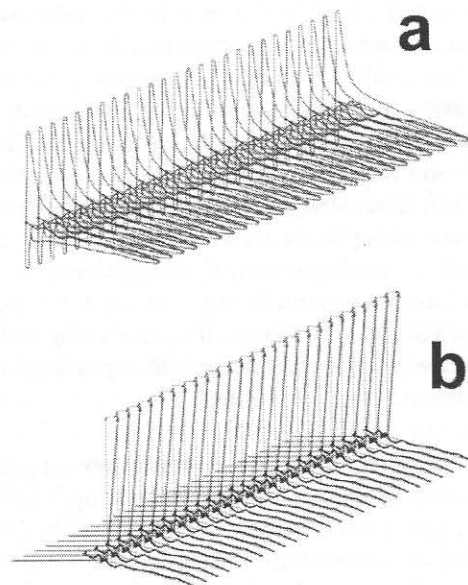
Figure 4. Here we have represented a dragonfly wing by showing a lot of cross sections spread over the length of the wing from base to tip (assuming the wing width or chord is constant and not tapered for now). We could envision this as representing the three dimensional pressure or force distribution over the entire wing. Fig. 4a shows the pressure distribution and Fig. 4b the force distribution over the wing.
