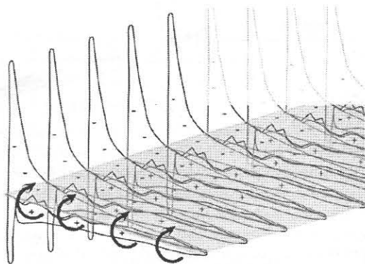
Figure 5. A close up of the tip of the wing with the pressure distribution represented as in Fig. 4. We can see that there is nothing separating the high pressure below the wing from the low pressure above the wing to the left of the wingtip, so there will be a flow of air from below to above the wing at the wingtip, lowering the pressure below the wing and increasing the pressure above the wing in the vicinity of the tip.
